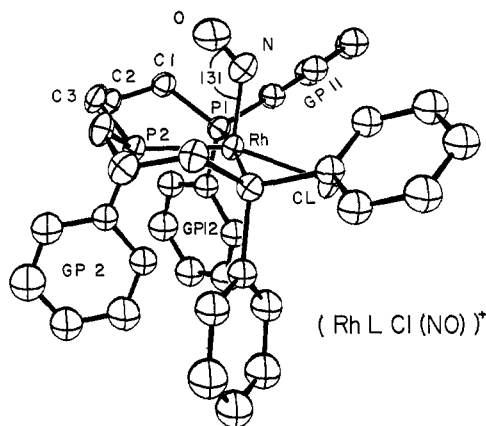
Figure 4. Perspective view of [RhLCl(NO)] + approximately down the y axis. Rh, P(2), Cl, N, and O lie on the mirror plane. The 50% probability ellipsoids are shown. Hydrogen atoms are not shown.
