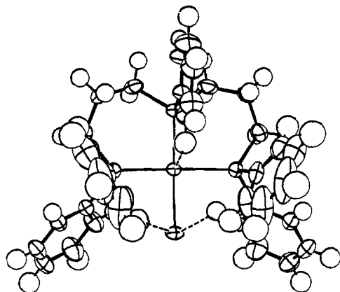
Figure 3. Perspective view of a single molecule of RhLCl showing the steric hindrance about a vacant axial coordination site. Close intramolecular contact distances are indicated by dotted lines. The 50% probability ellipsoids are shown with the hydrogen atoms as open circles. This is a view from the opposite direction of Figure 2.
