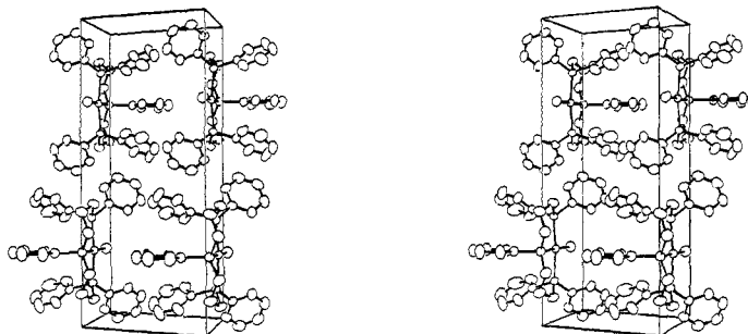
Figure 5. Stereoscopic view approximately down the z axis with the outline of one unit cell of RhLCl indicated. Hydrogen atoms are not shown.
